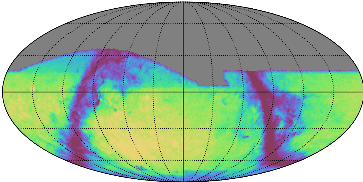
baseline_v2.0_10yrs g: GalaxyCountsMetricExtended
