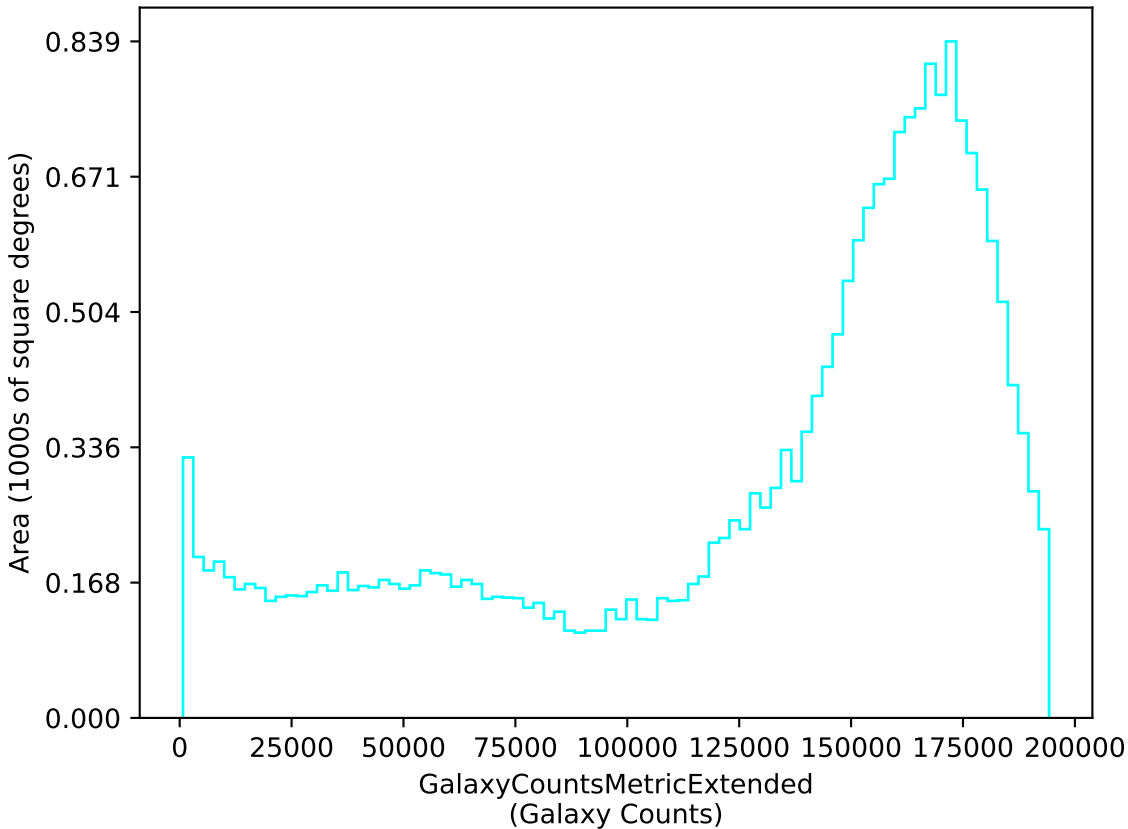
baseline_v2.0_10yrs u: GalaxyCountsMetricExtended
