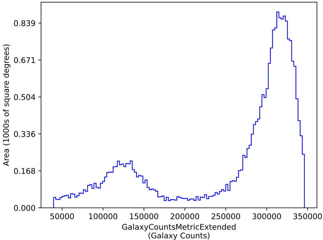
baseline_v2.0_10yrs y: GalaxyCountsMetricExtended
