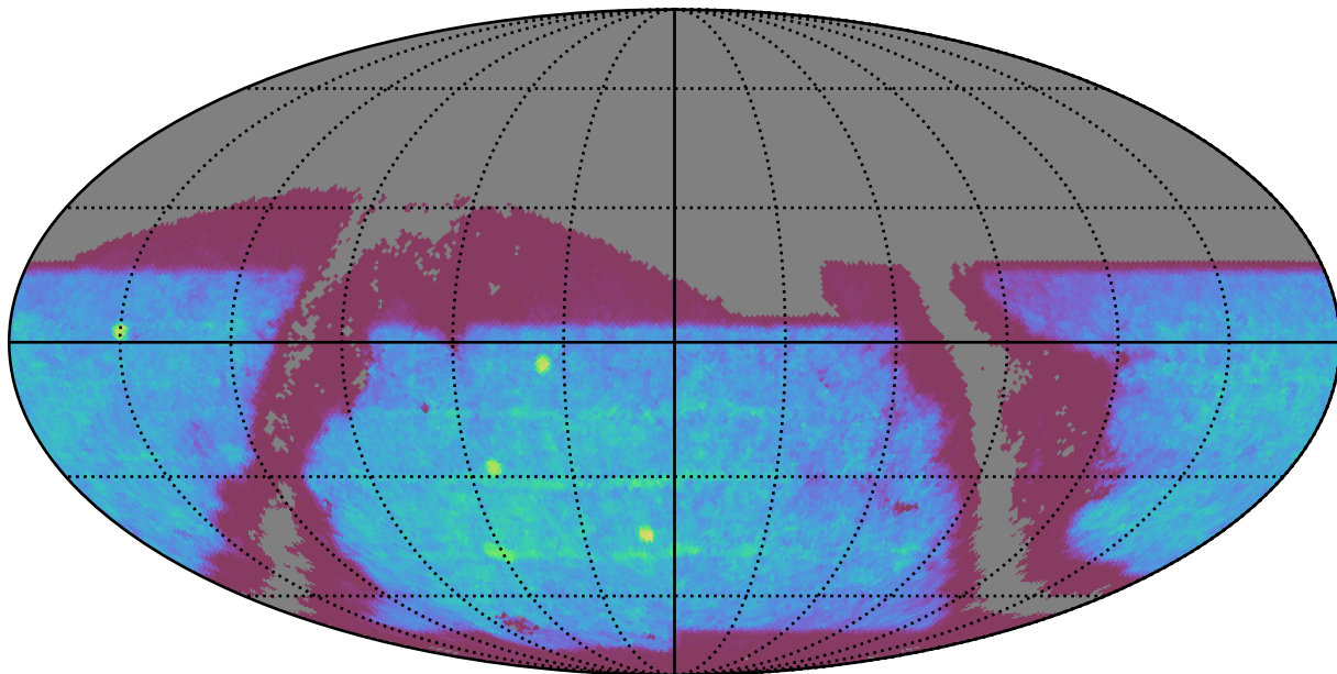
baseline_v2.0_10yrs : SNSLMetric
