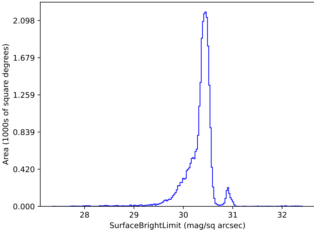
baseline_v2.0_10yrs g: SurfaceBrightLimit
