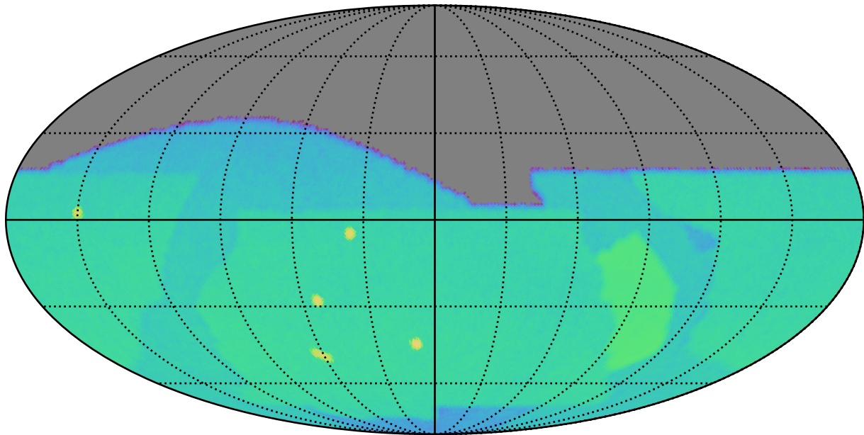
baseline_v2.0_10yrs g: SurfaceBrightLimit
