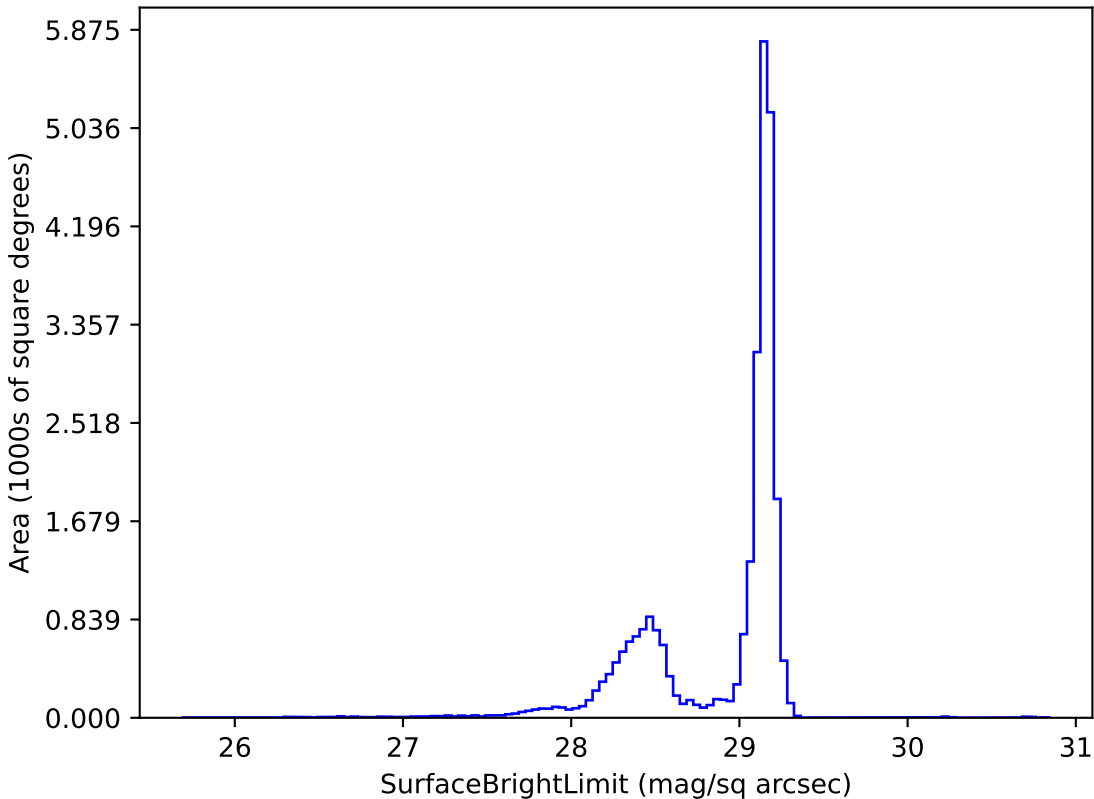
baseline_v2.0_10yrs z: SurfaceBrightLimit
