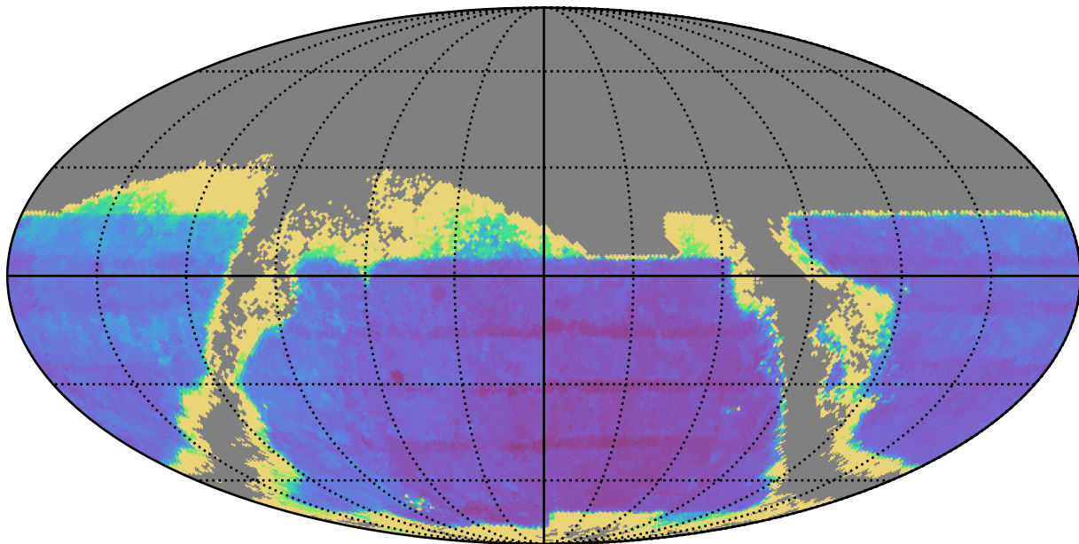
baseline_v2.0_10yrs : TDC_accuracy
