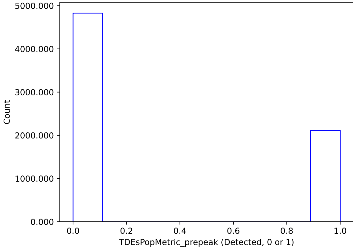
baseline_v2.0_10yrs : TDEsPopMetric_prepeak
