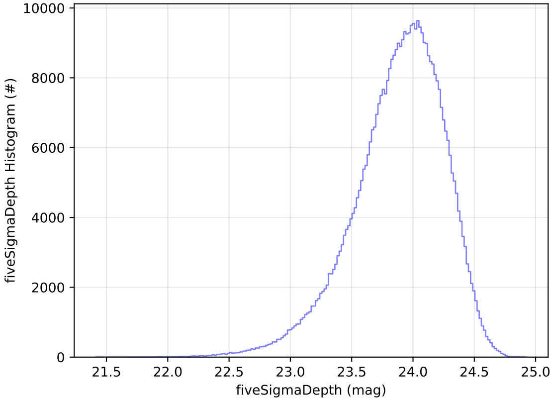
baseline_v2.0_10yrs r: fiveSigmaDepth Histogram
