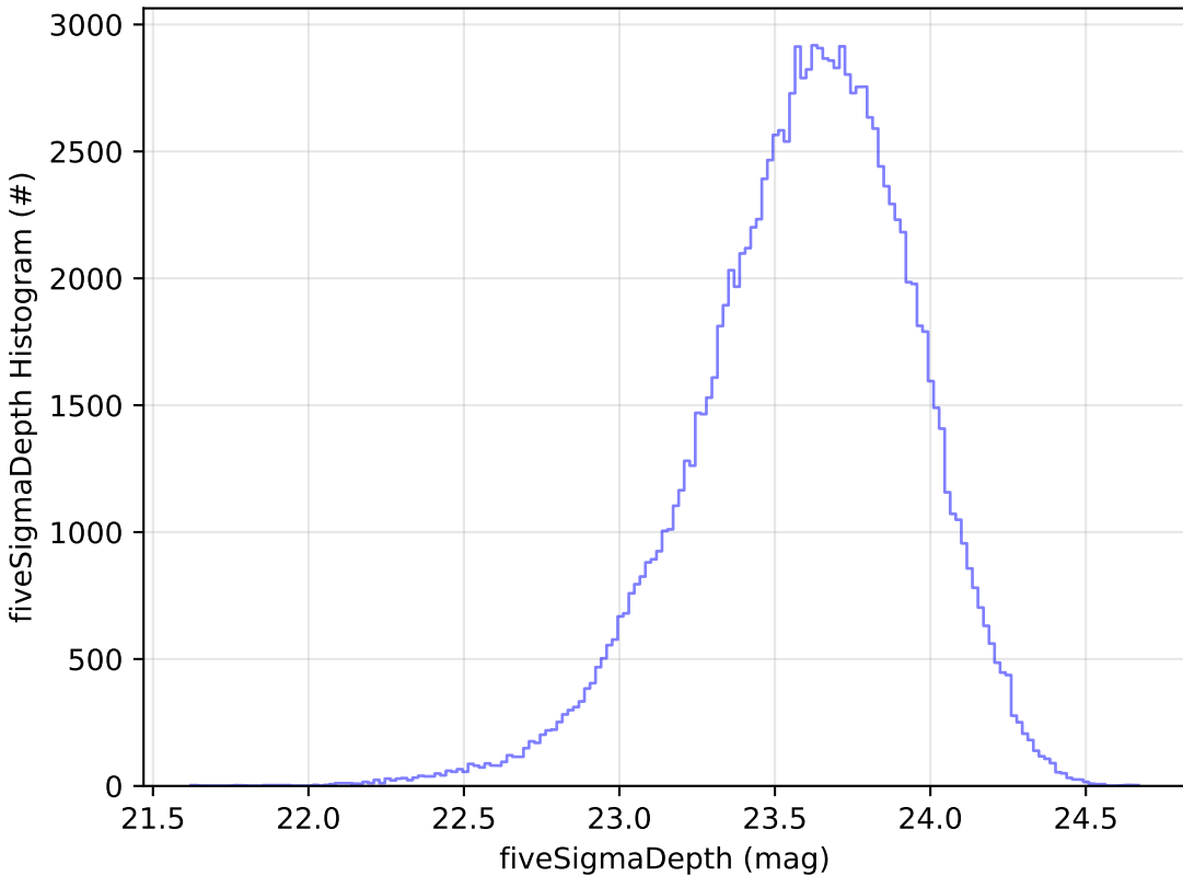
baseline_v2.0_10yrs u: fiveSigmaDepth Histogram
