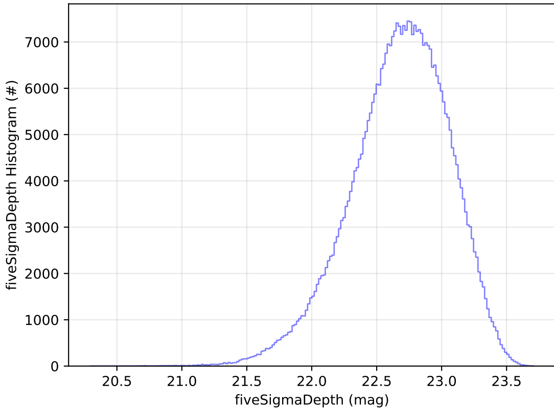
baseline_v2.0_10yrs z: fiveSigmaDepth Histogram
