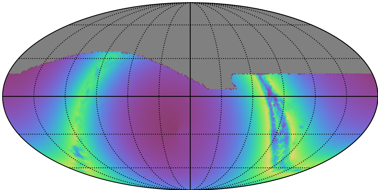
baseline_v2.0_10yrs : young_stars
