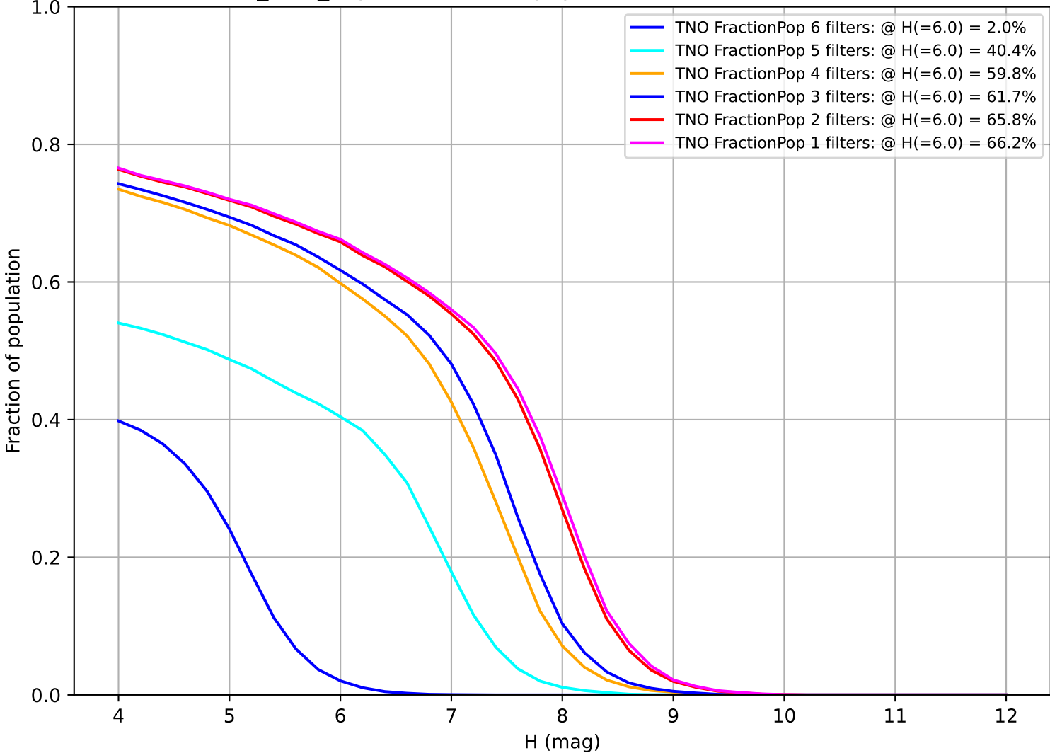
baseline_v2.0_10yrs: Fraction of population with colors in X filters TNO
