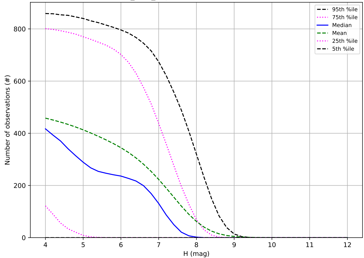
baseline_v2.0_10yrs: Number of observations TNO
