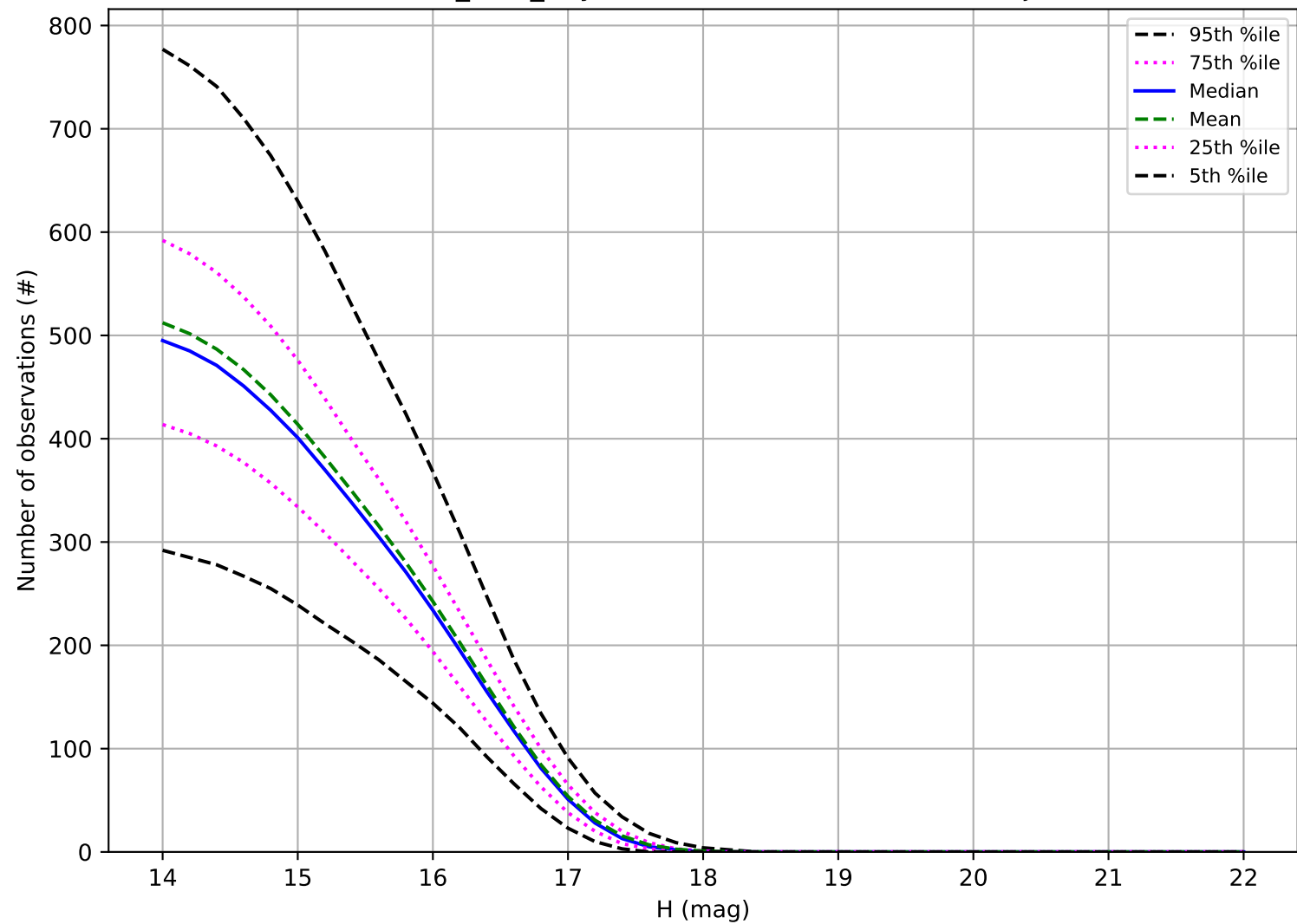
baseline_v2.0_10yrs: Number of observations Trojan
