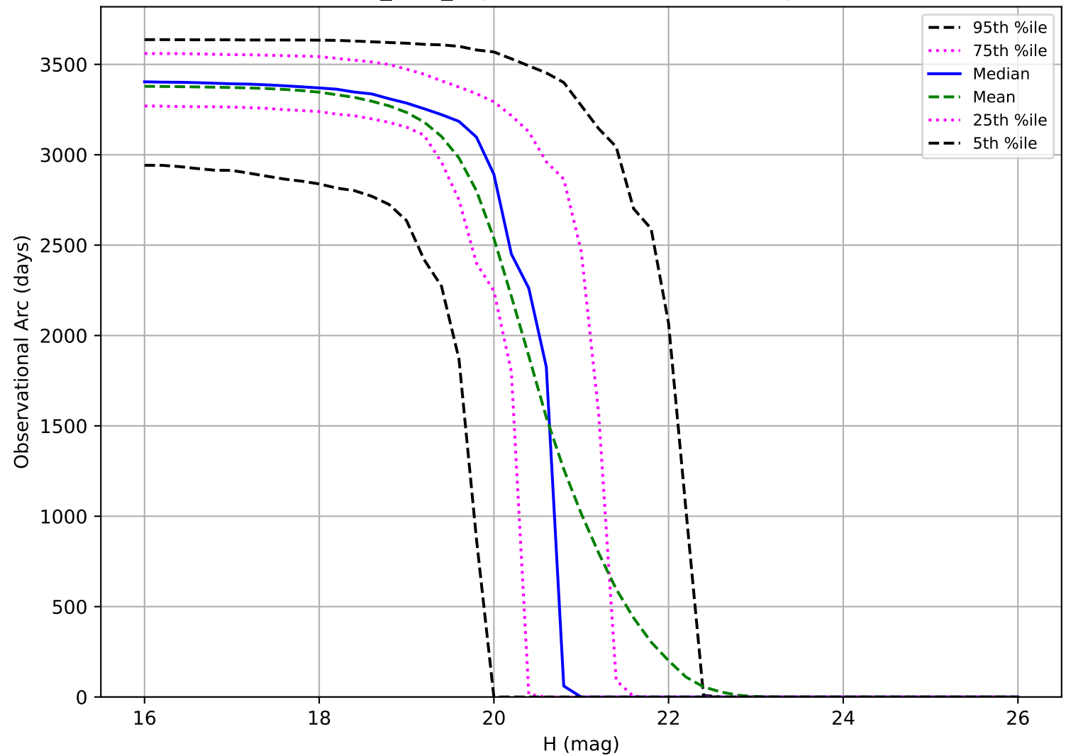
baseline_v2.0_10yrs: Observational Arc Length MBA
