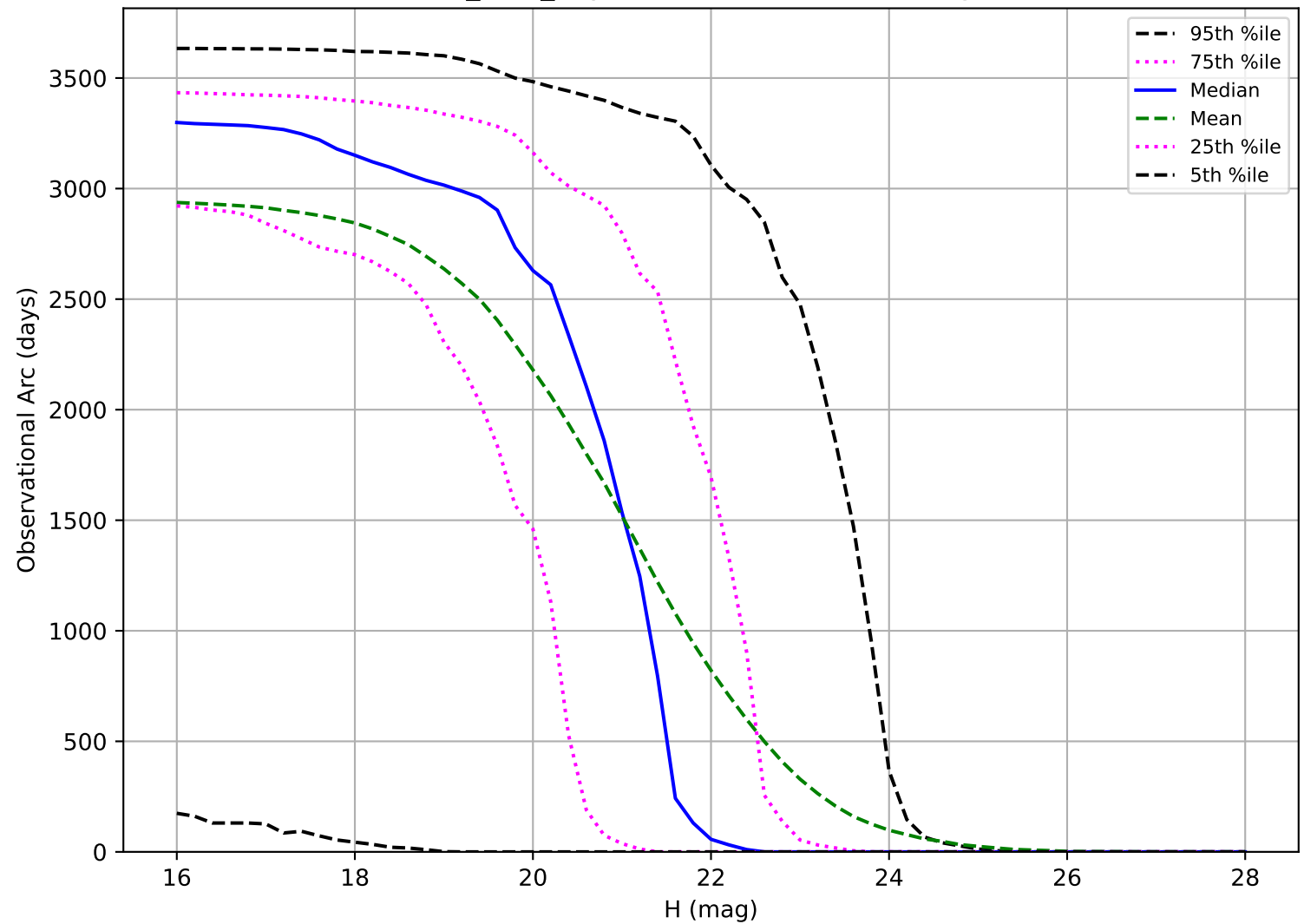
baseline_v2.0_10yrs: Observational Arc Length NEO
