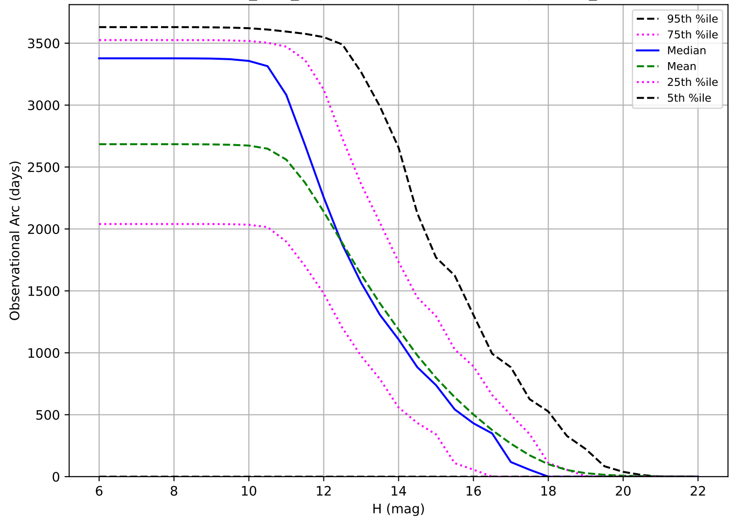
baseline_v2.0_10yrs: Observational Arc Length OCC_r5
