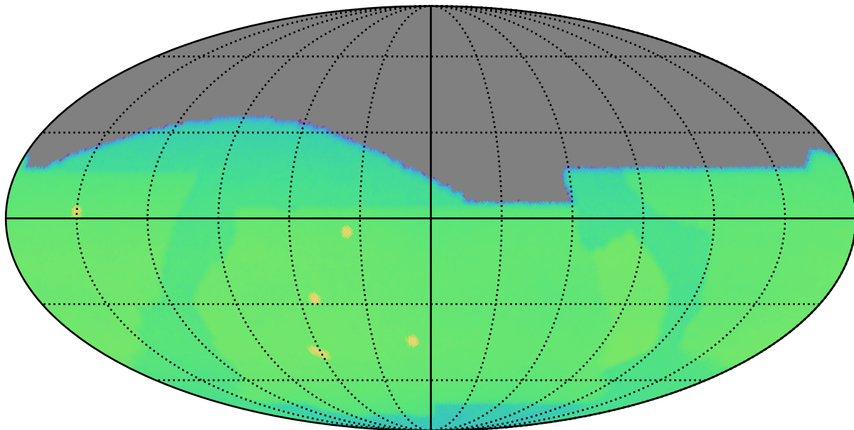
baseline_v2.1_10yrs : CoaddM5
