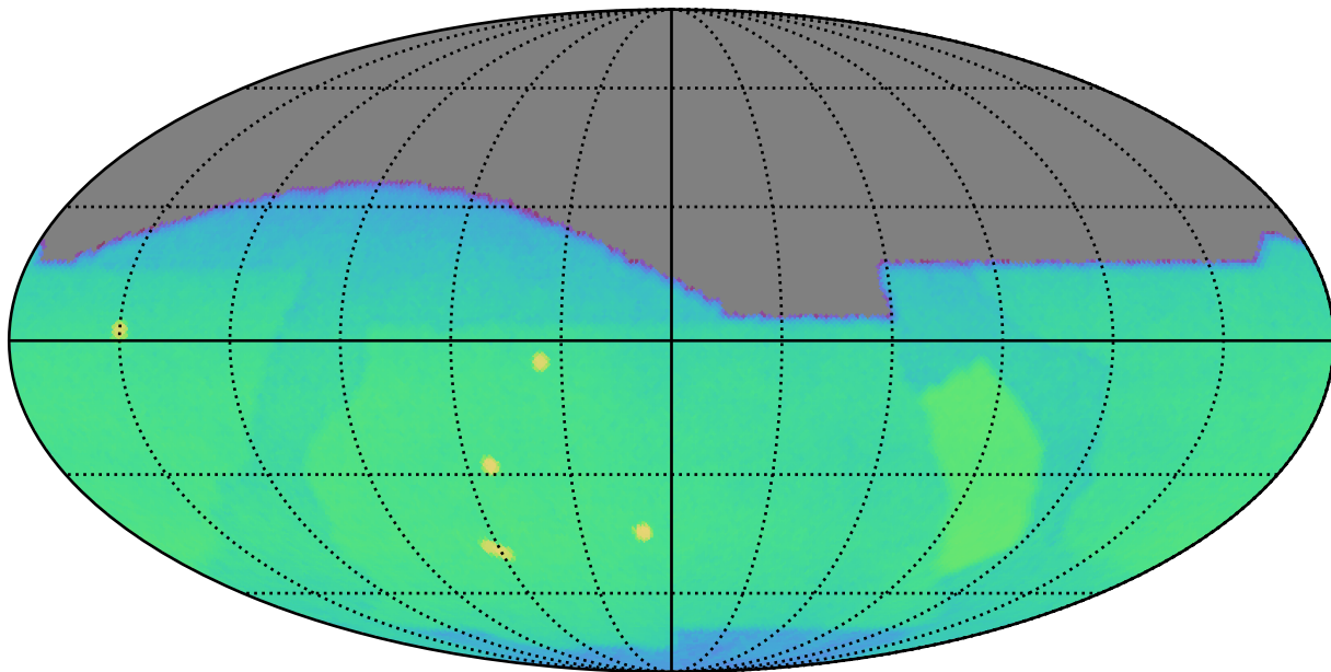
baseline_v2.1_10yrs g: CoaddM5
