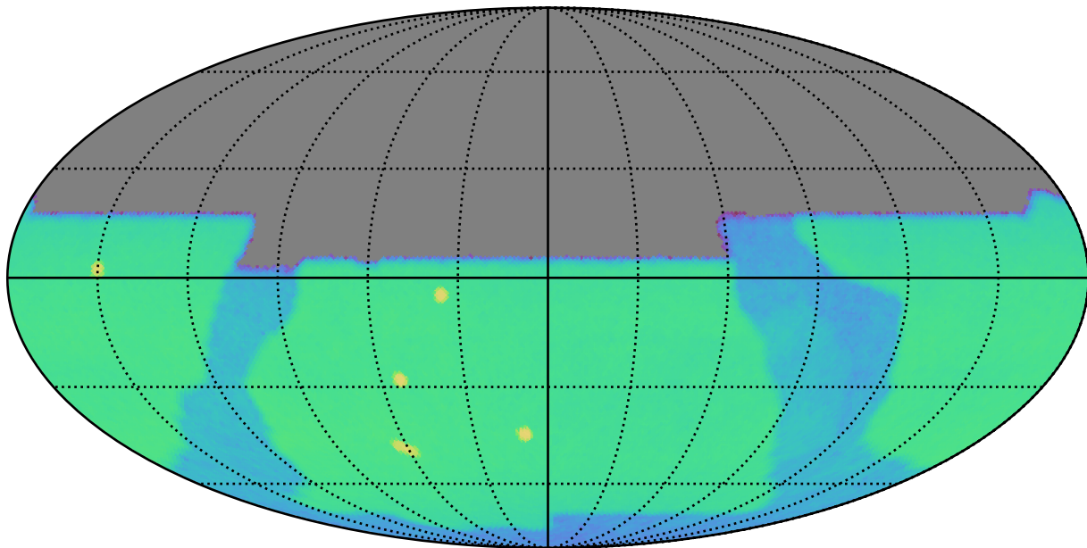
baseline_v2.1_10yrs y: CoaddM5
