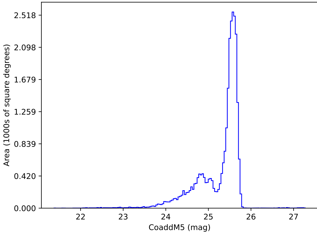
baseline_v2.1_10yrs z: CoaddM5
