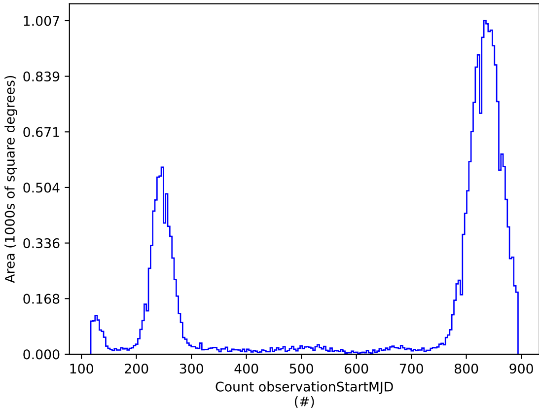
baseline_v2.1_10yrs : Count observationStartMJD
