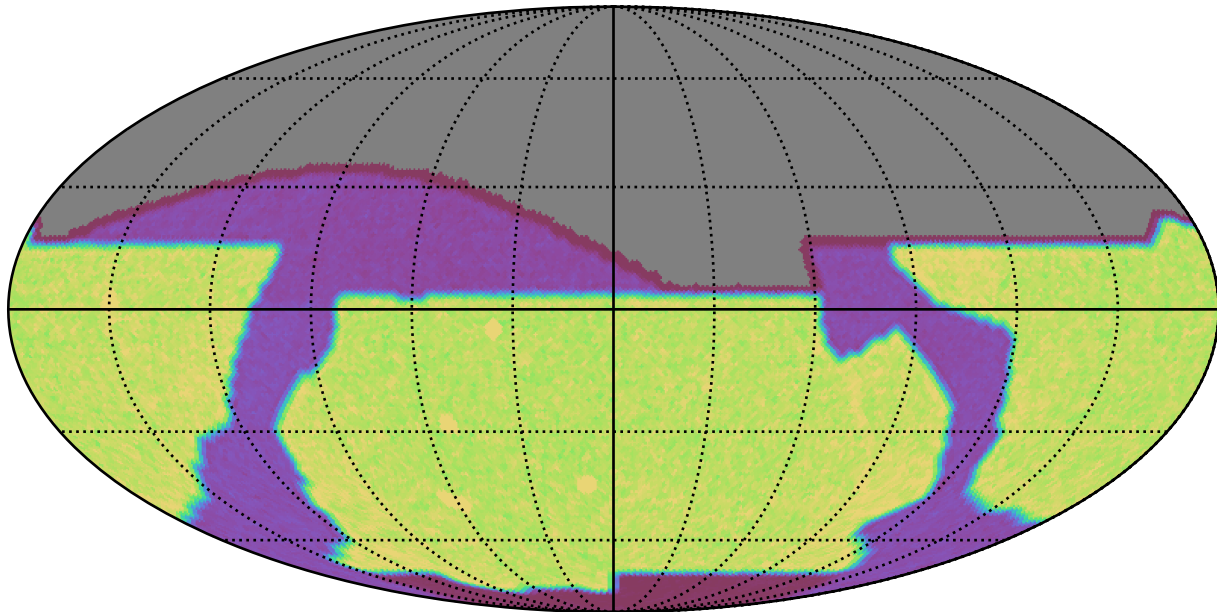
baseline_v2.1_10yrs : Count observationStartMJD
