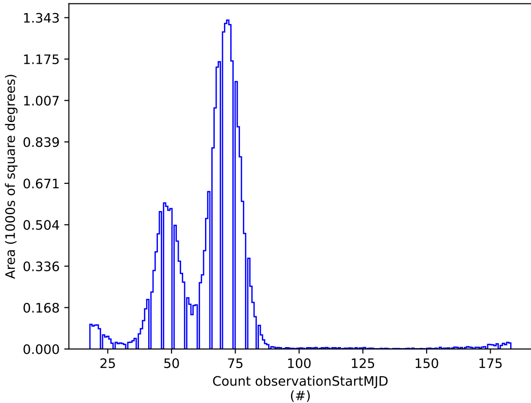
baseline_v2.1_10yrs g: Count observationStartMJD
