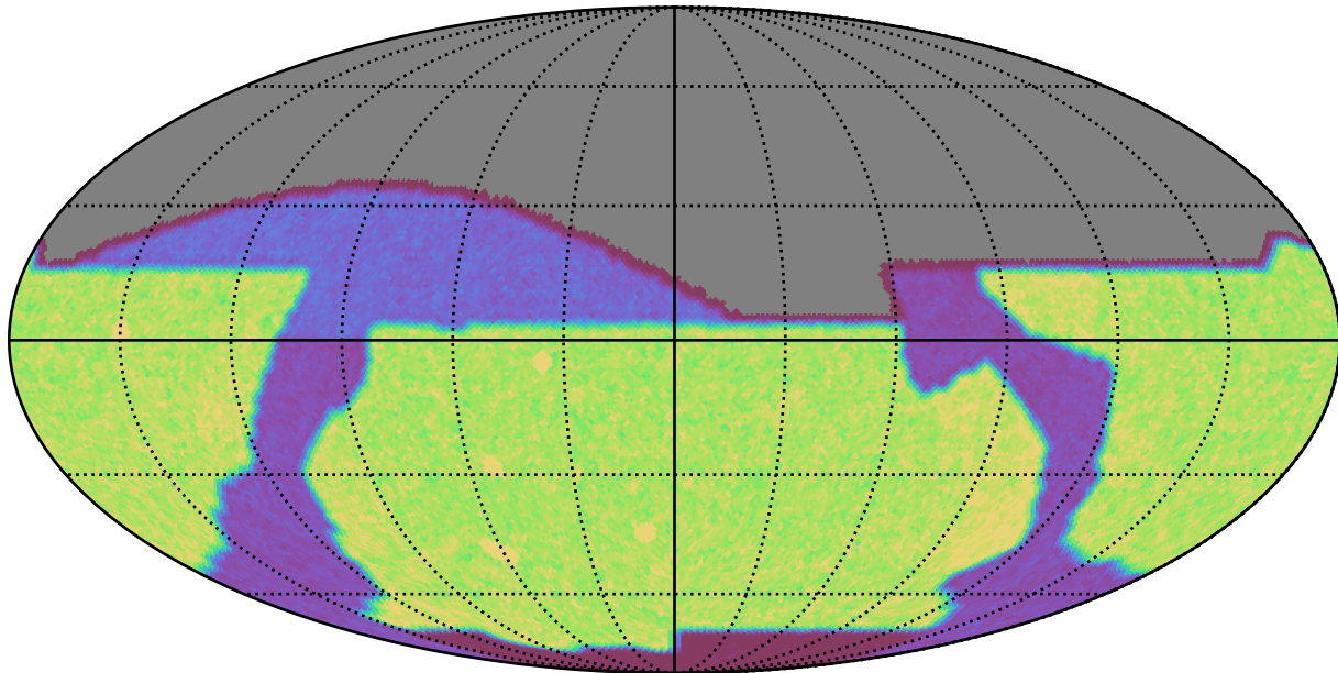
baseline_v2.1_10yrs i: Count observationStartMJD
