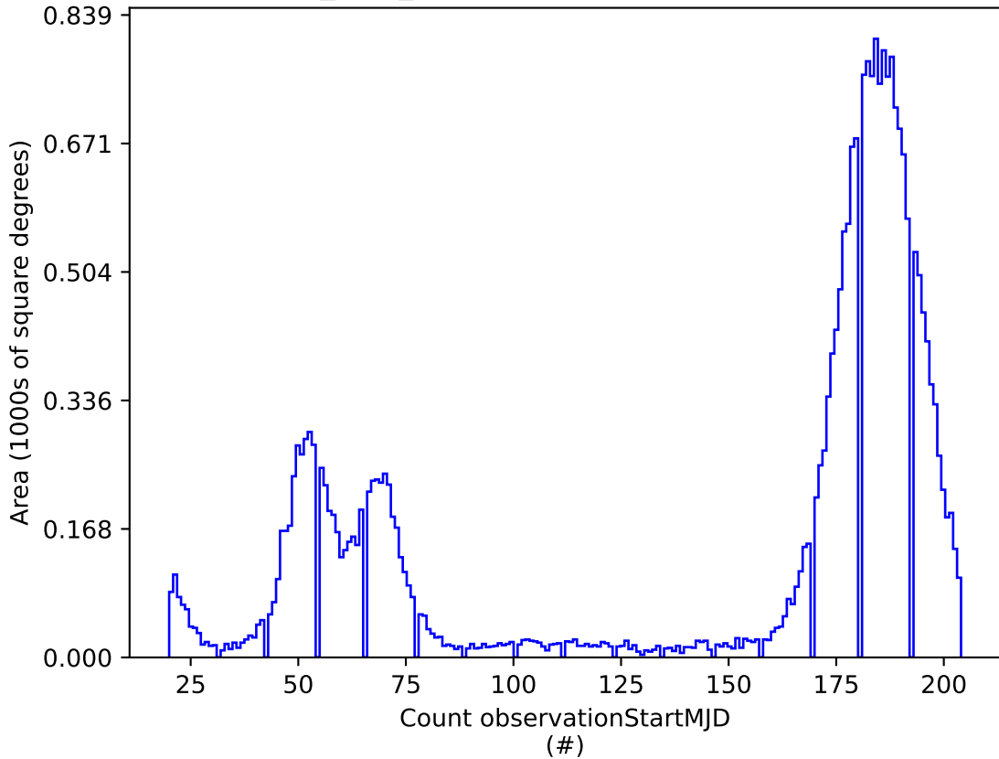
baseline_v2.1_10yrs r: Count observationStartMJD
