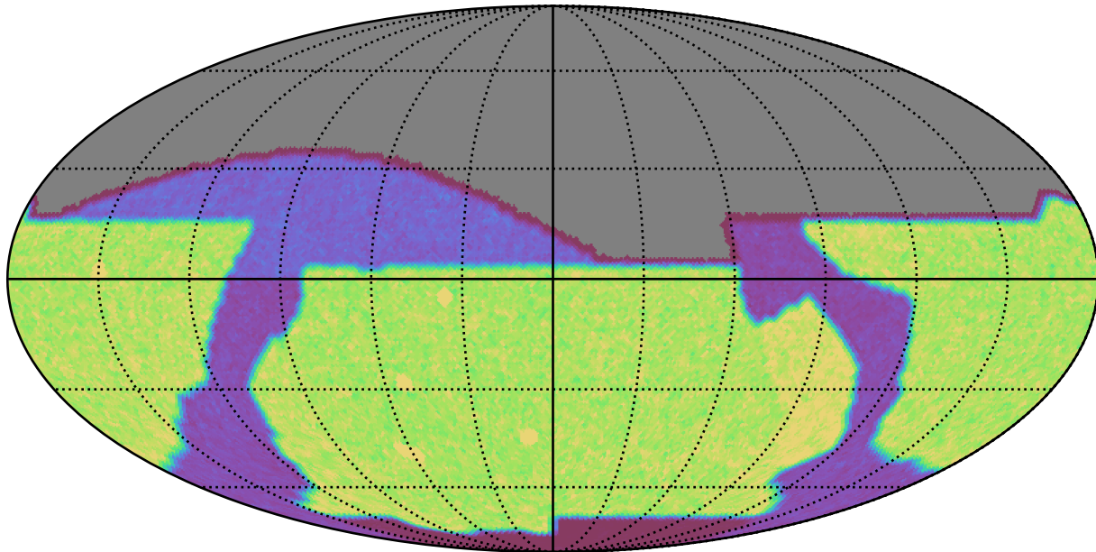
baseline_v2.1_10yrs r: Count observationStartMJD
