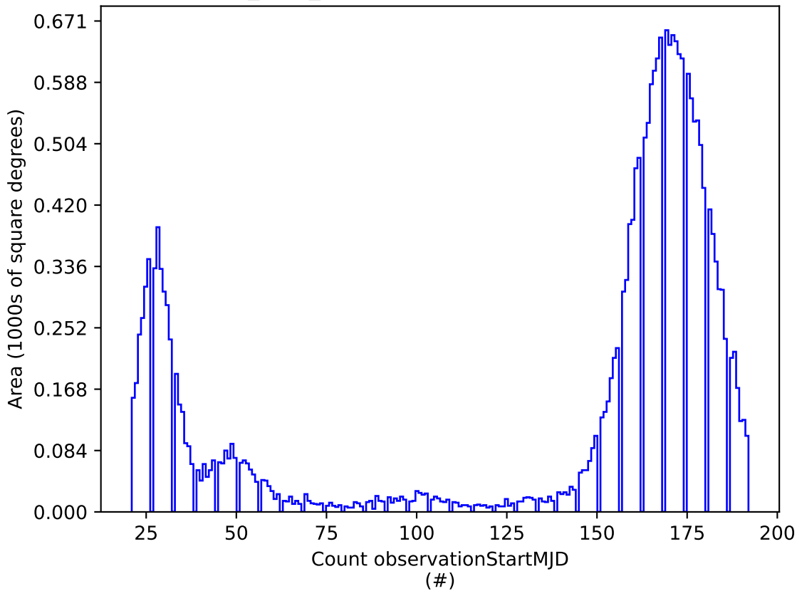
baseline_v2.1_10yrs y: Count observationStartMJD
