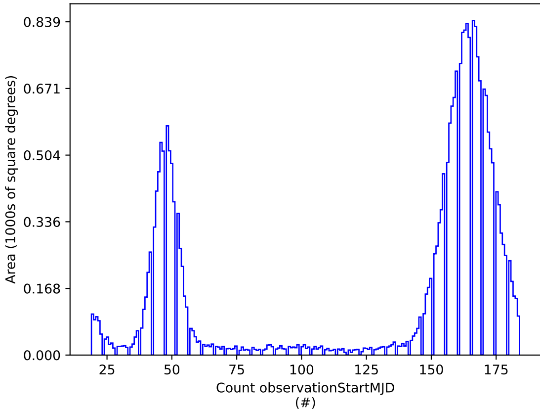
baseline_v2.1_10yrs z: Count observationStartMJD
