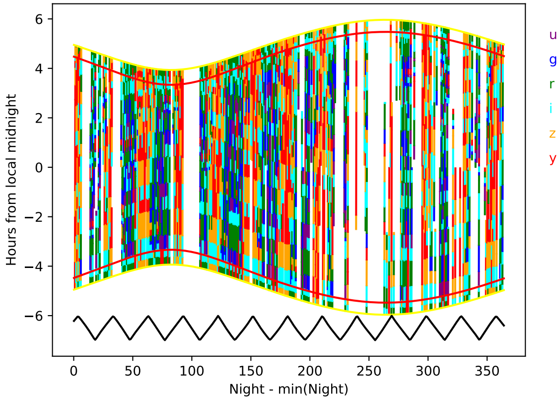
baseline_v2.1_10yrs year 5-6: Hourglass
