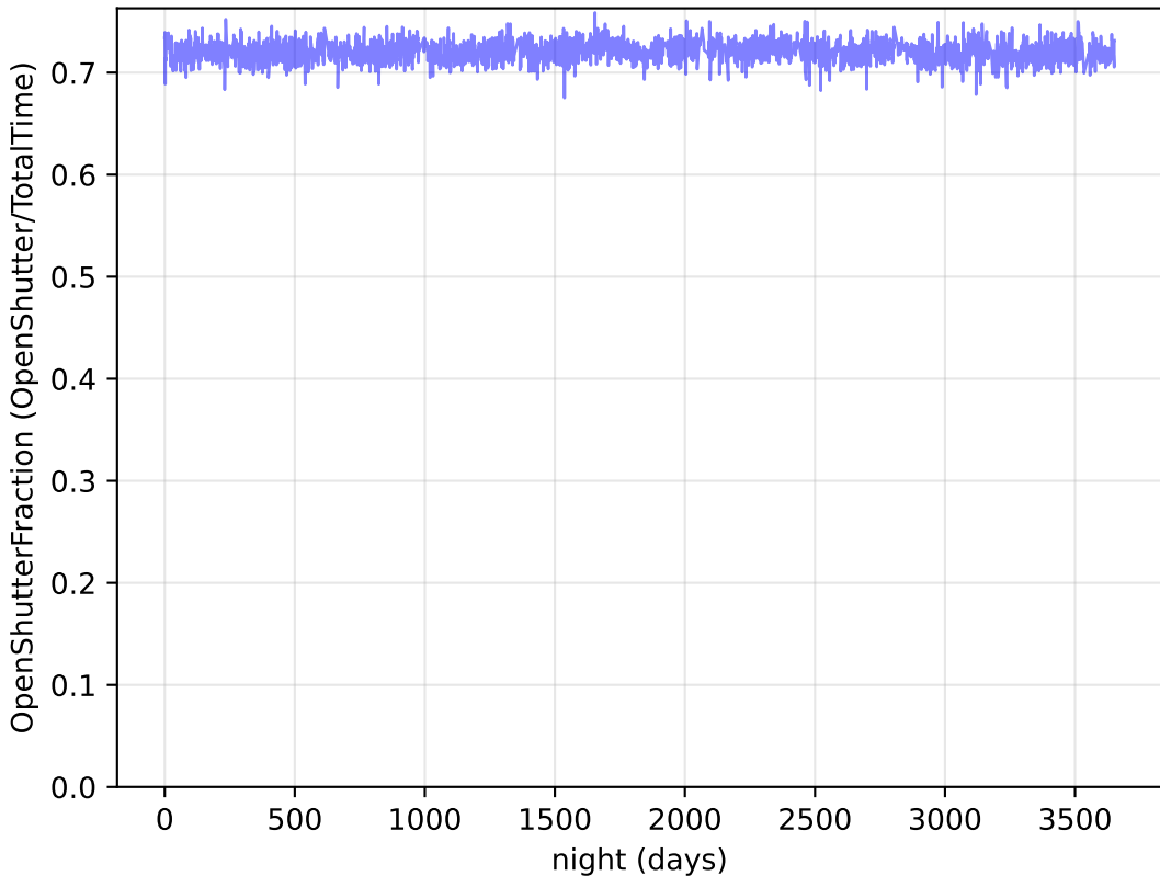
baseline_v2.1_10yrs : OpenShutterFraction
