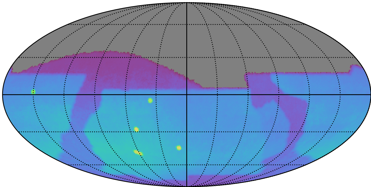
baseline_v2.1_10yrs : Brown Dwarf, L7
