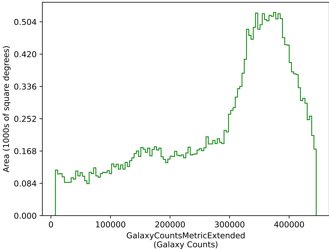
baseline_v2.1_10yrs g: GalaxyCountsMetricExtended
