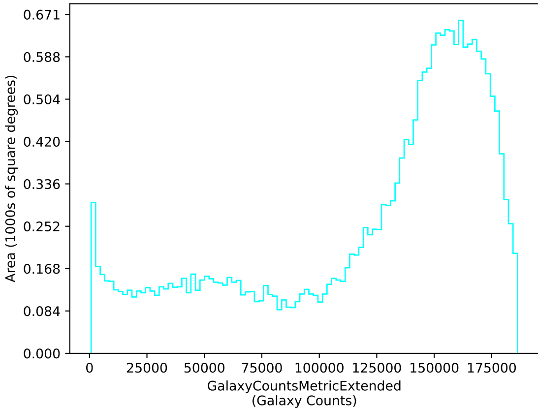
baseline_v2.1_10yrs u: GalaxyCountsMetricExtended
