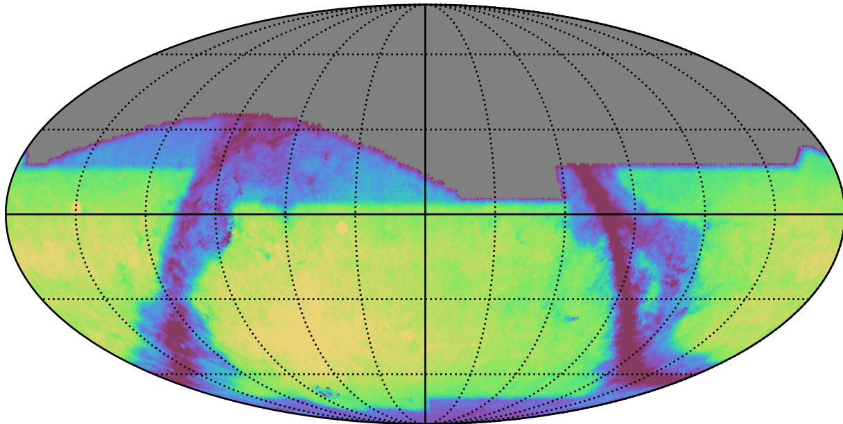
baseline_v2.1_10yrs z: GalaxyCountsMetricExtended
