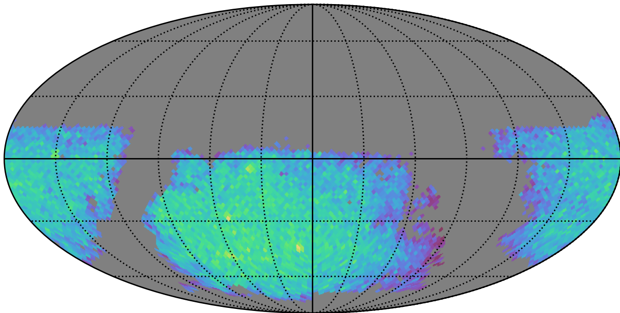
baseline_v2.1_10yrs gi: LVDwarfs
