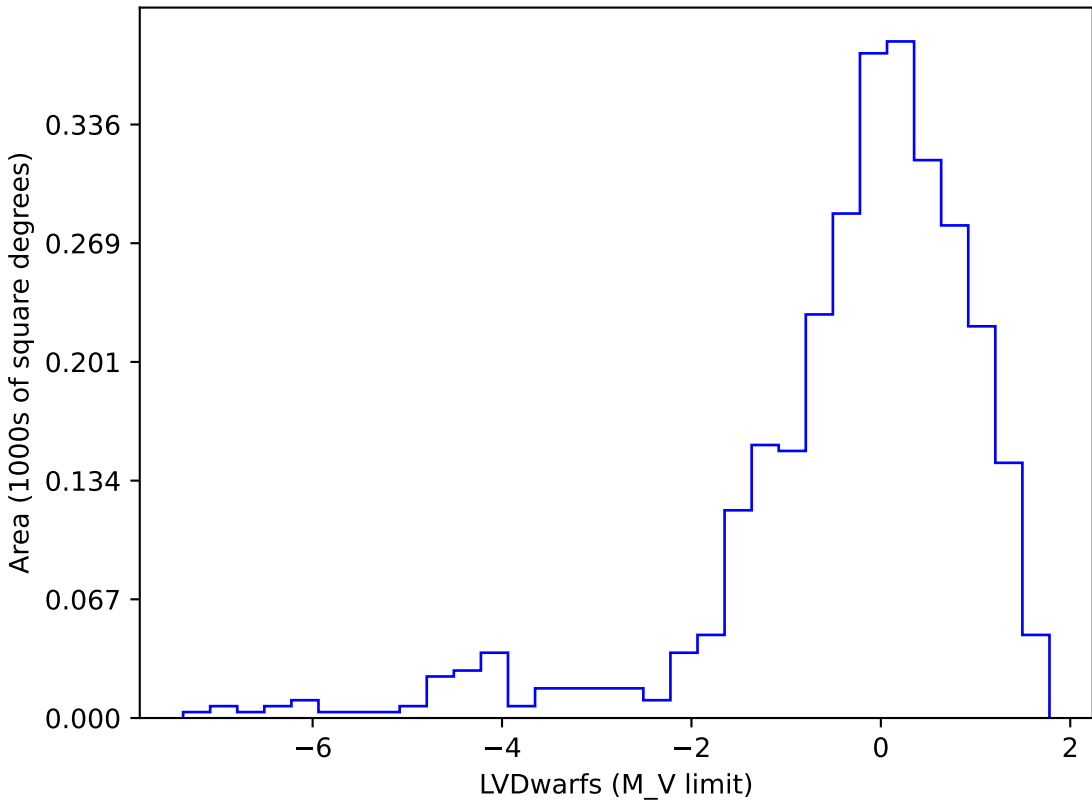
baseline_v2.1_10yrs gi SCP: LVDwarfs
