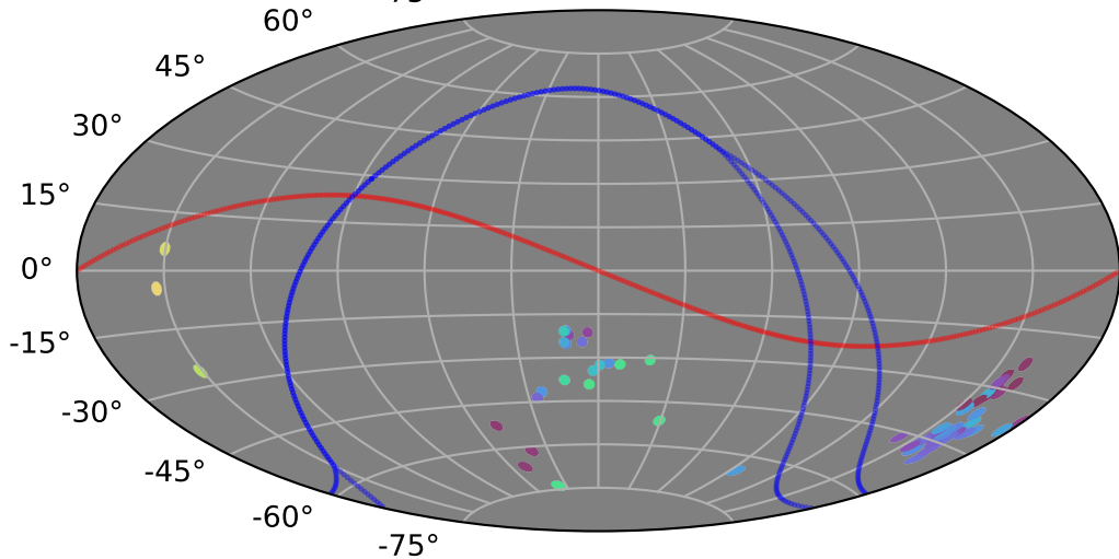
baseline_v2.1_10yrs gi: LVDwarfs 75°
