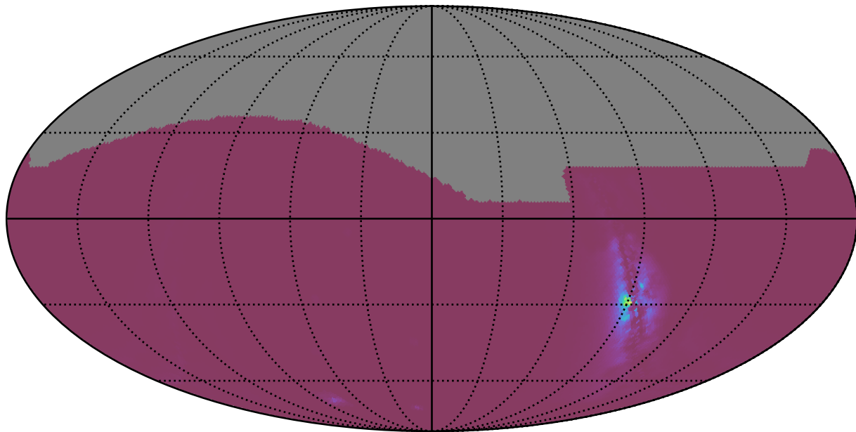
baseline_v2.1_10yrs : NlcPoints
