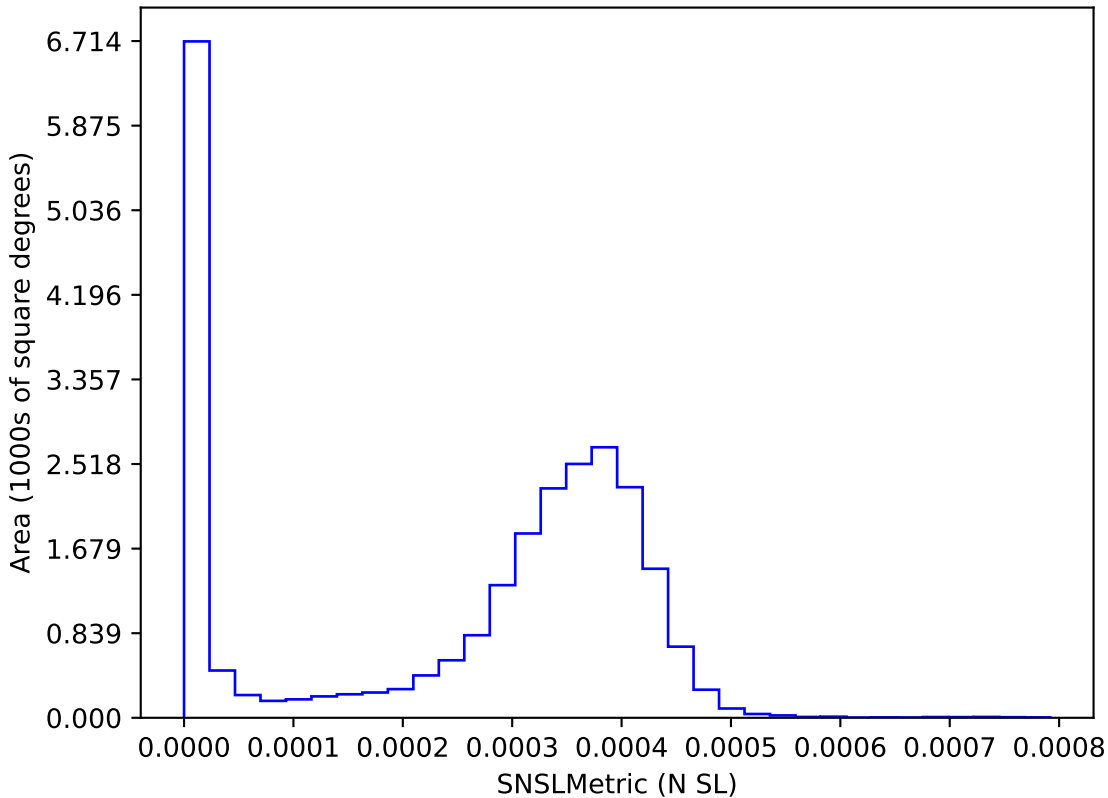
baseline_v2.1_10yrs : SNSLMetric
