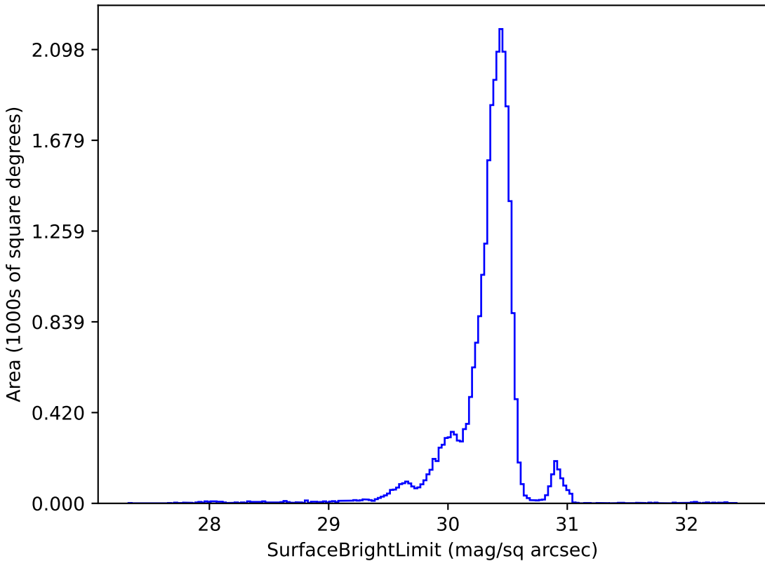
baseline_v2.1_10yrs g: SurfaceBrightLimit
