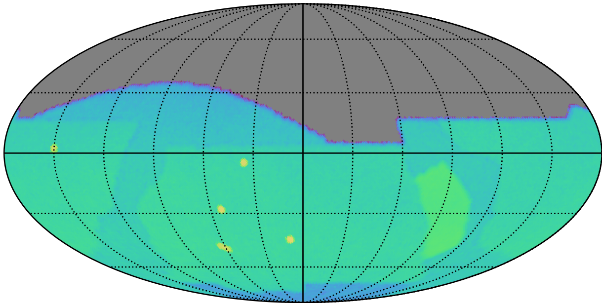
baseline_v2.1_10yrs g: SurfaceBrightLimit
