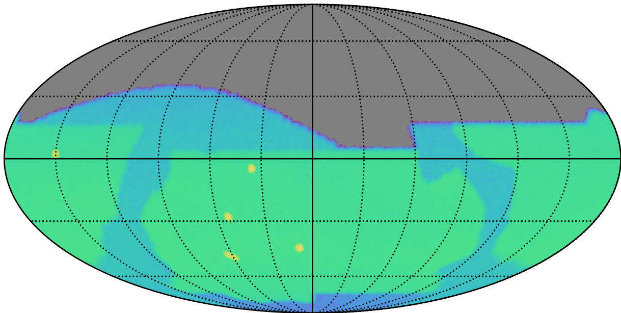
baseline_v2.1_10yrs r: SurfaceBrightLimit
