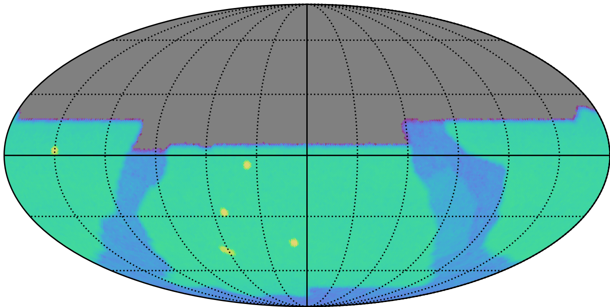
baseline_v2.1_10yrs y: SurfaceBrightLimit
