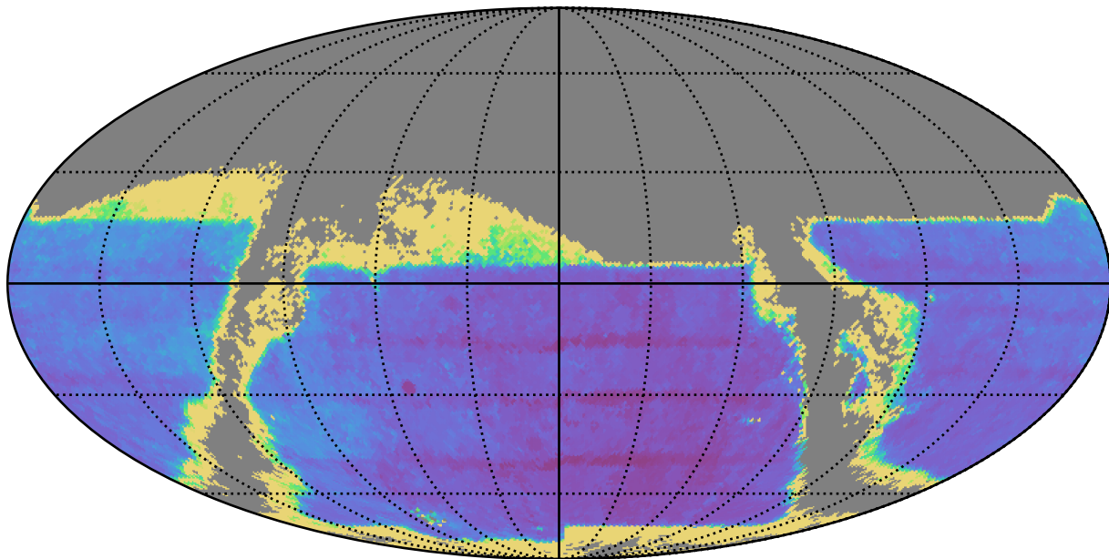
baseline_v2.1_10yrs : TDC_accuracy
