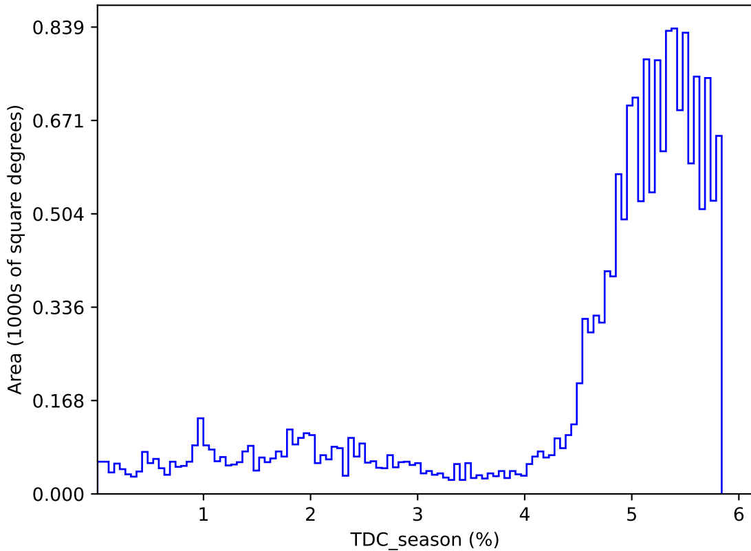
baseline_v2.1_10yrs : TDC_season
