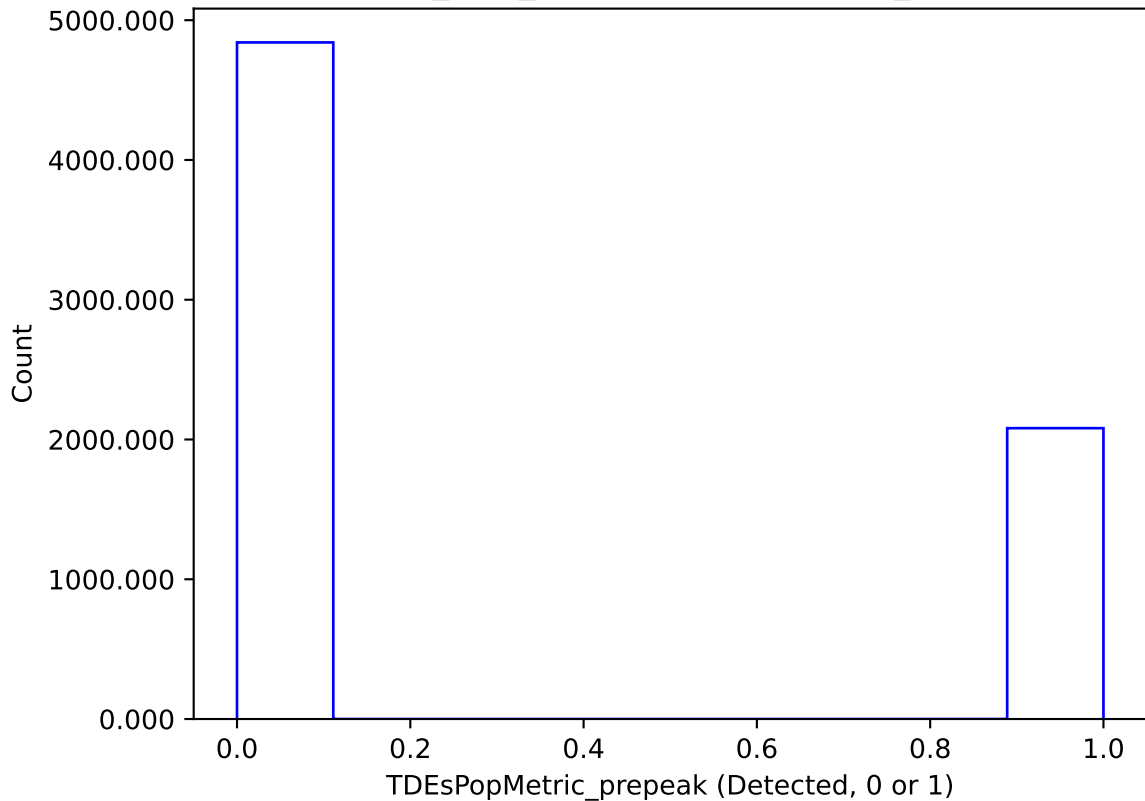
baseline_v2.1_10yrs : TDEsPopMetric_prepeak
