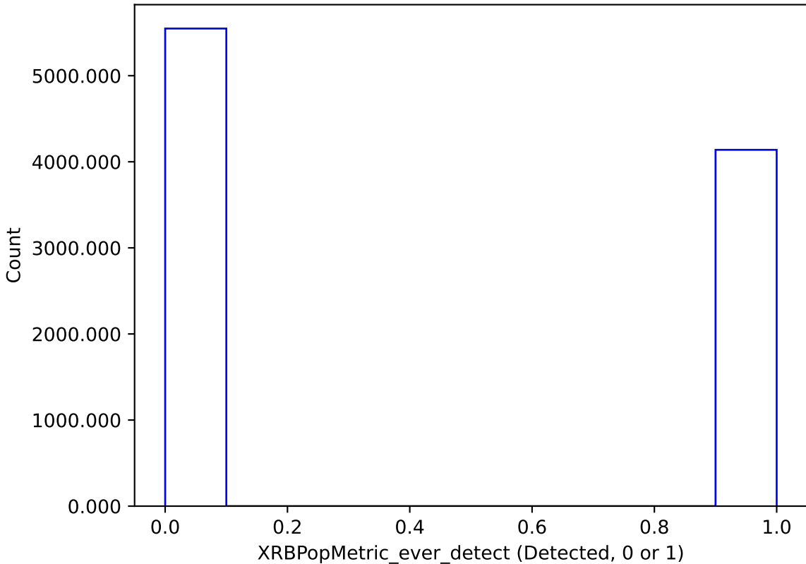
baseline_v2.1_10yrs : XRBPoMetric_ever_detect
